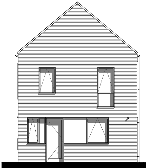
Rear Elevation
