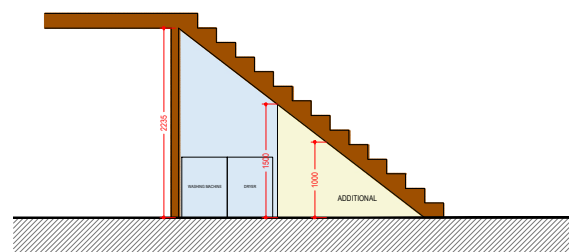
STAIR SECTION (UNDER STAIR STORAGE)
