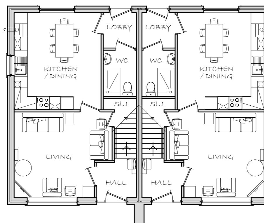
GF Plan-Type "F1"
