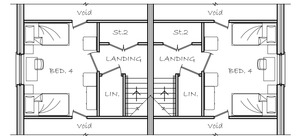
SF Plan-Type "F1"
