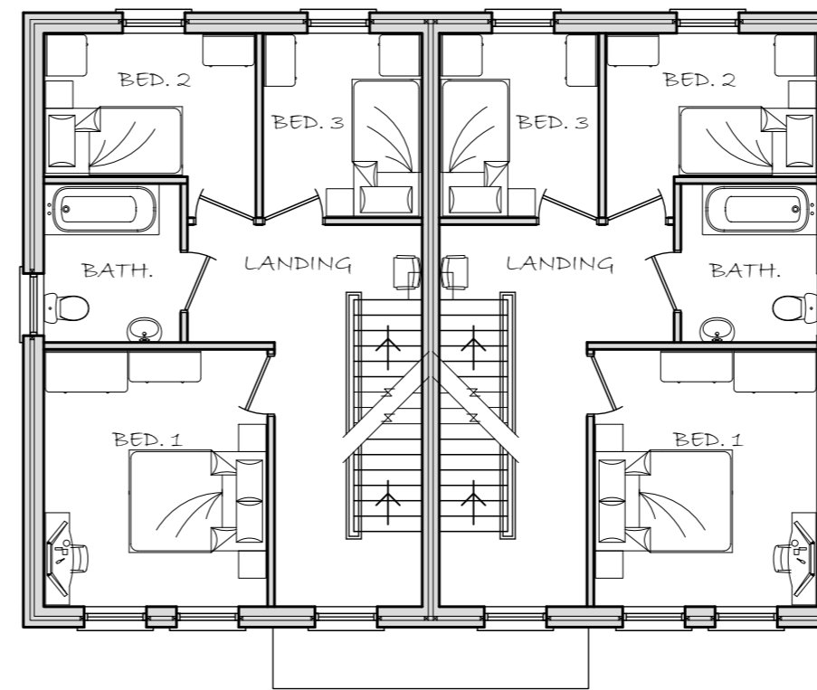
FF Plan-Type "F1"
