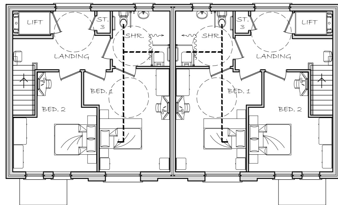
FF Plan-Type "A2" wc
