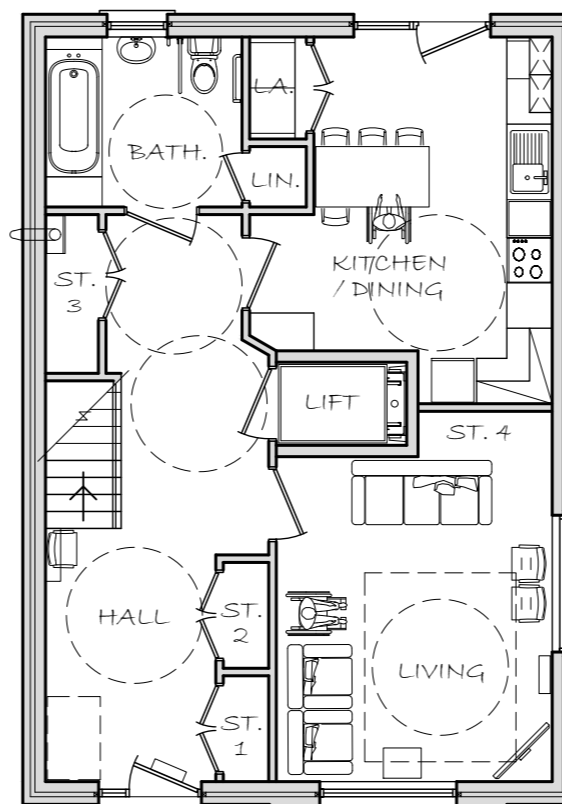
GF Plan-Type "E2" wc
