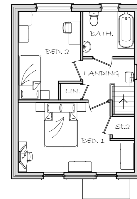
FF Plan-Type "C1"
