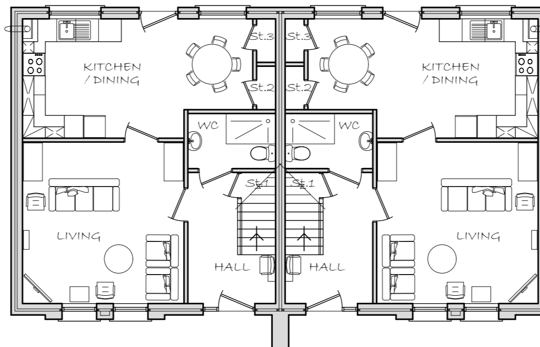
GF Plan-Type "B1"
