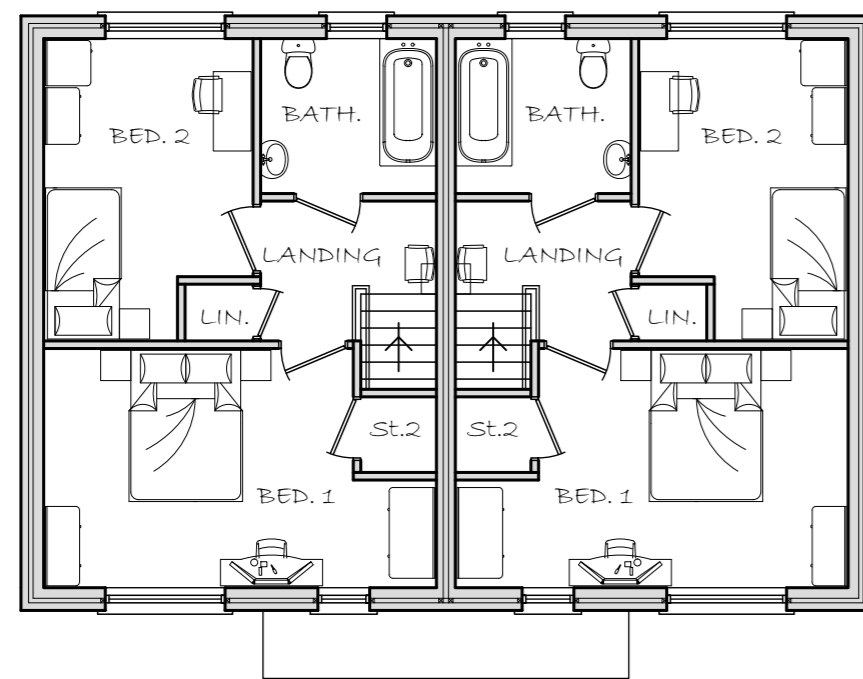
FF Plan-Type "A1"
