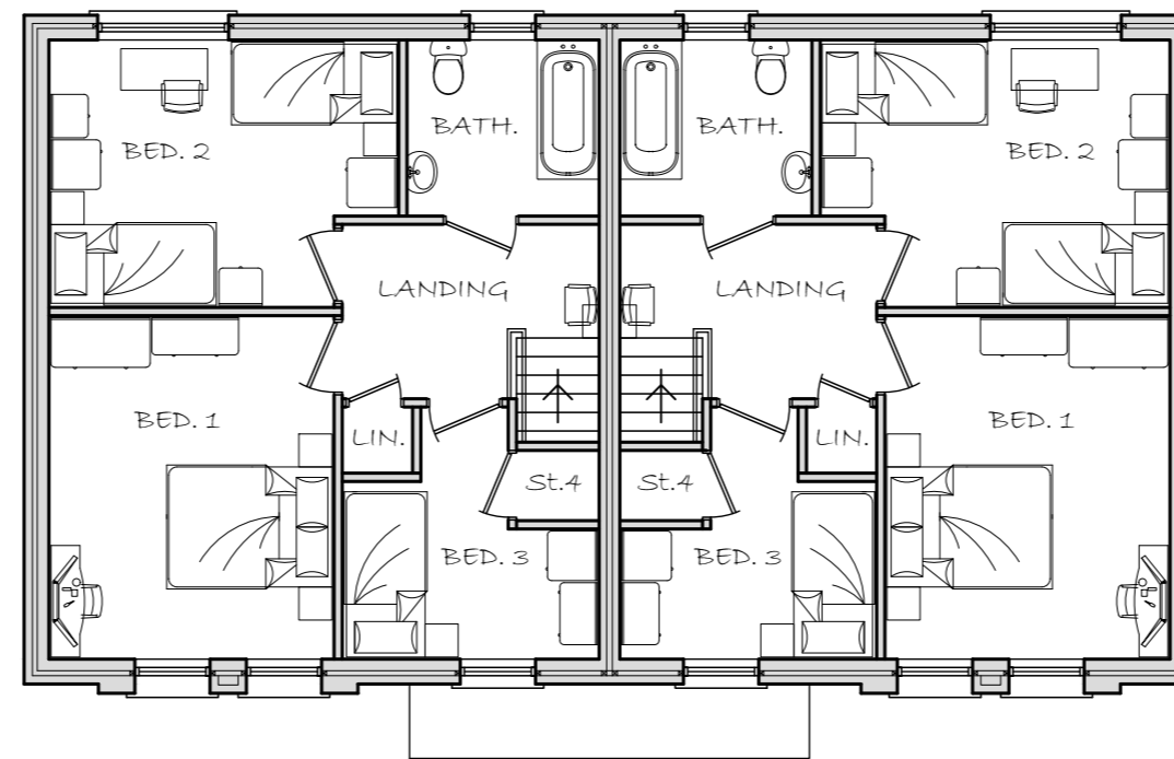
FF Plan-Type "B1"
