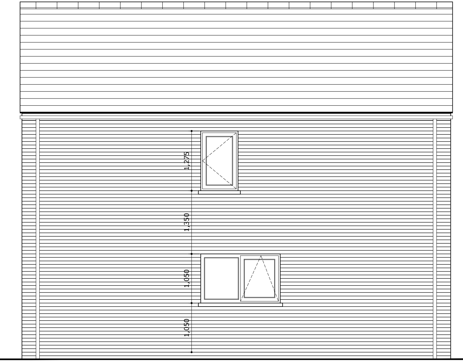
plot 1 : side elevation
