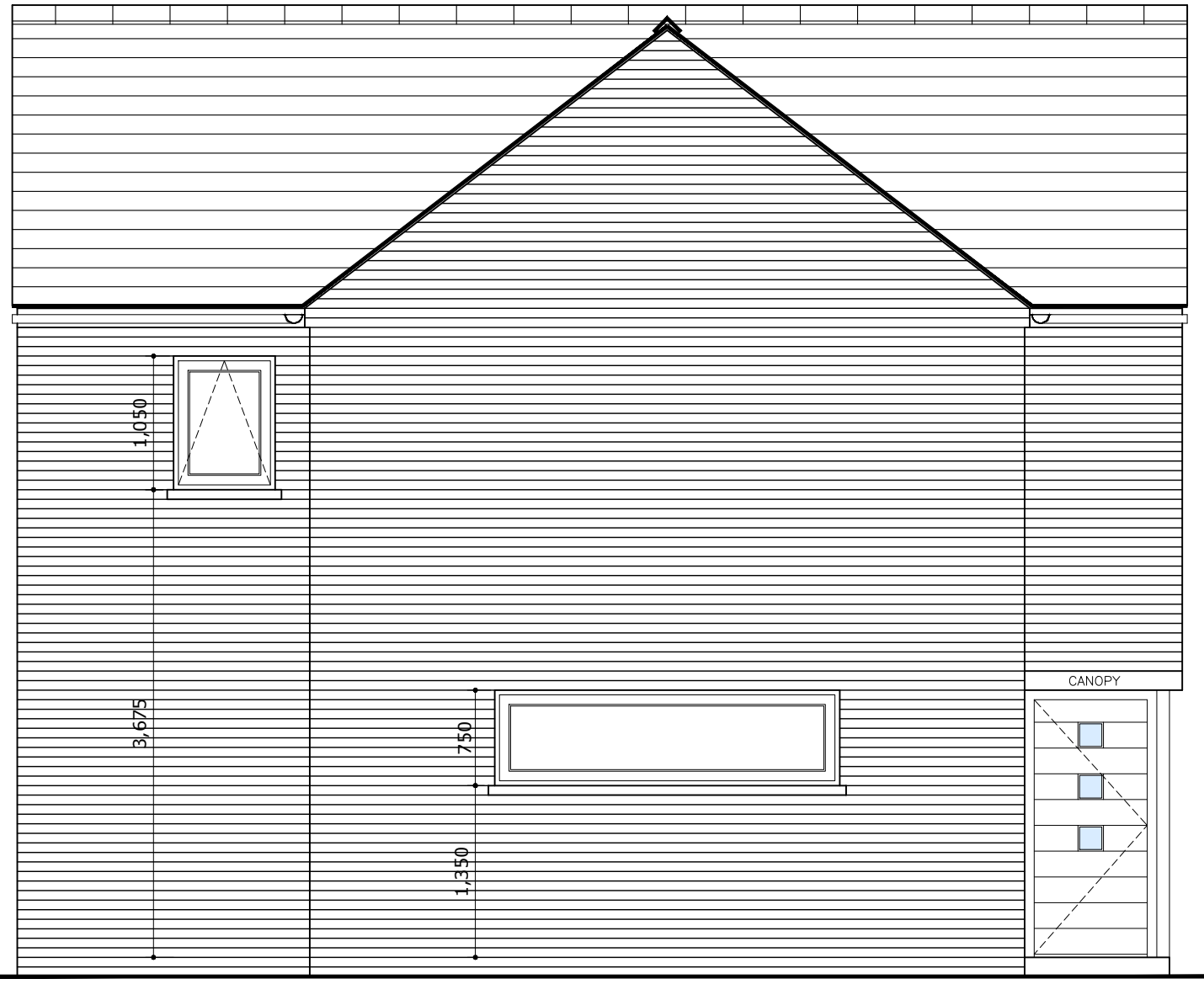
plot 1 : side elevation
