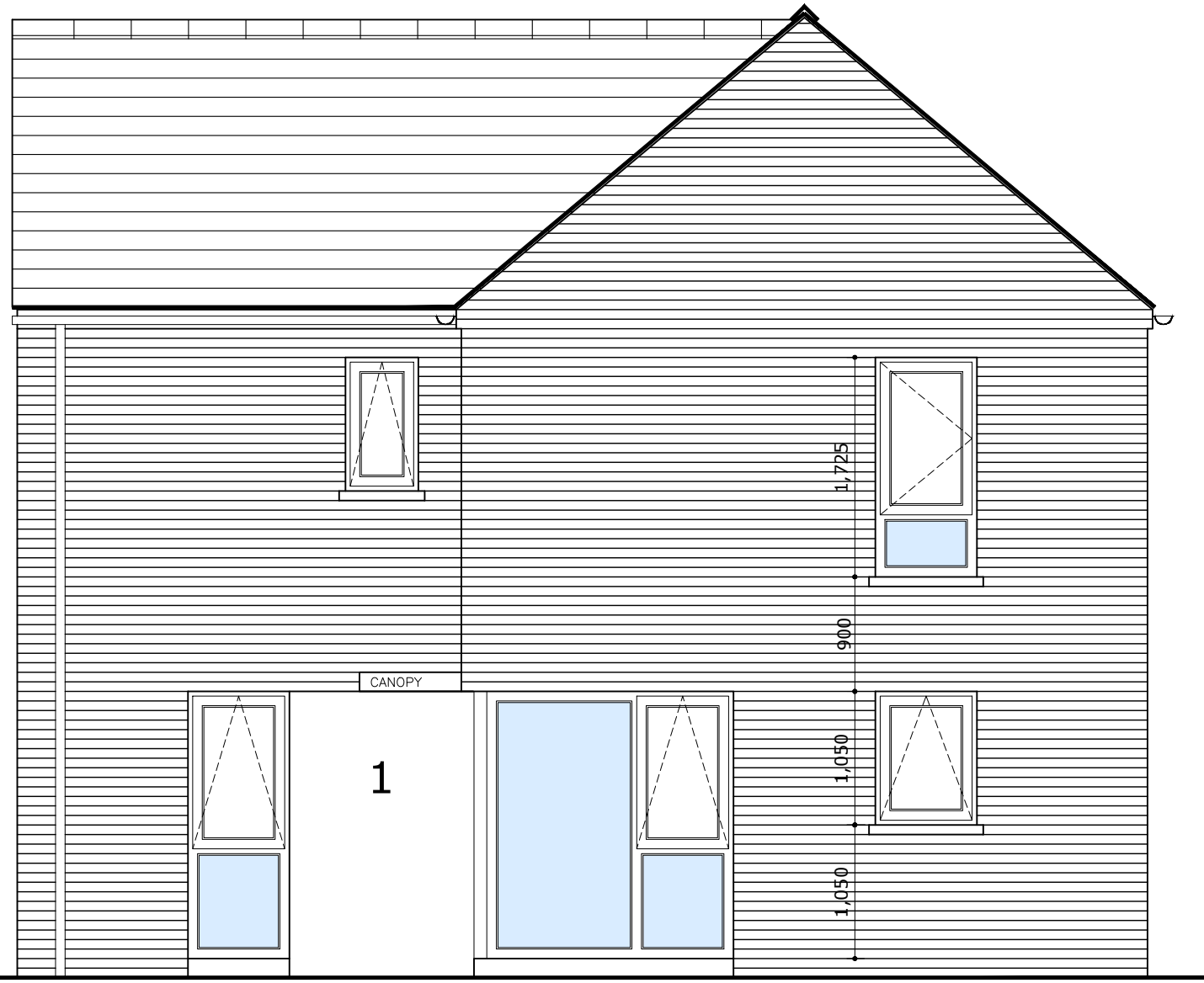
plot 1 : front elevation
